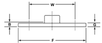
771 Companion Flange C – Cast
