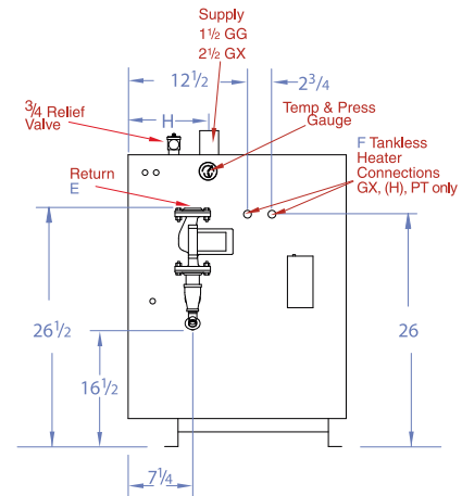
RIGHT SIDE VIEW GG and GXH PT Water Models
