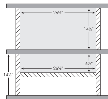
16" On-Center Framing
