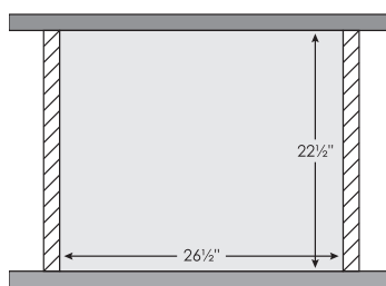
24" On-Center Framing
